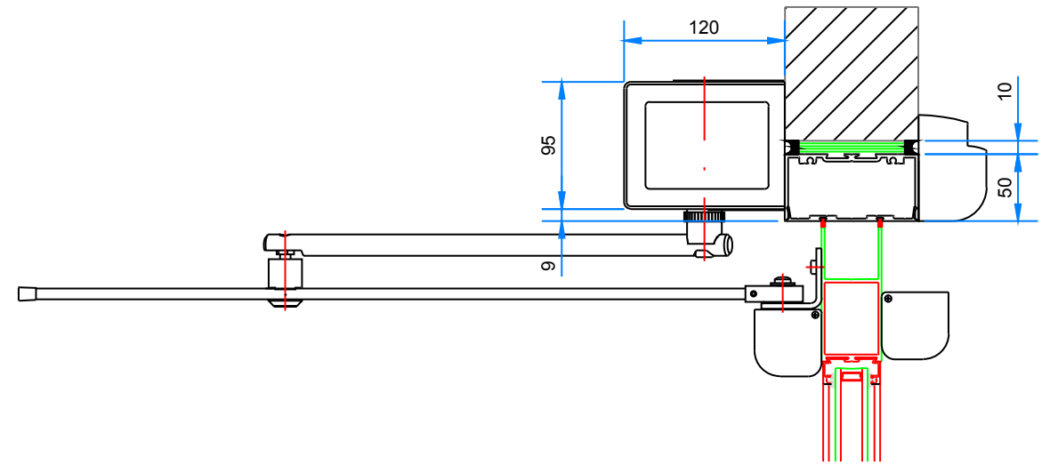
Outswing Rod Push Arm (50mm Section)
