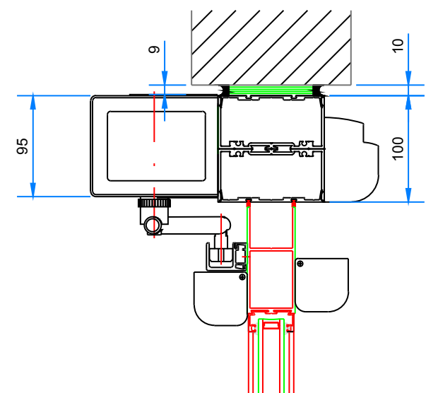
Outswing Tracked Push Arm (100mm Section)
