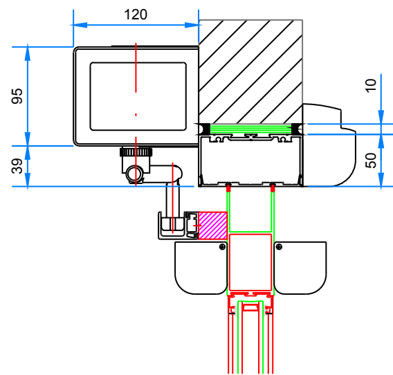
Inswing Tracked Pull Arm (50mm Section)
