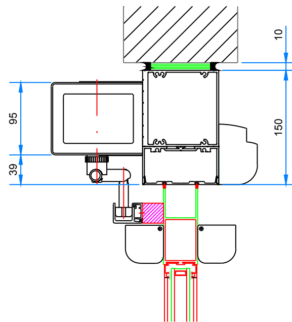
Inswing Tracked Pull Arm (150mm Section)
