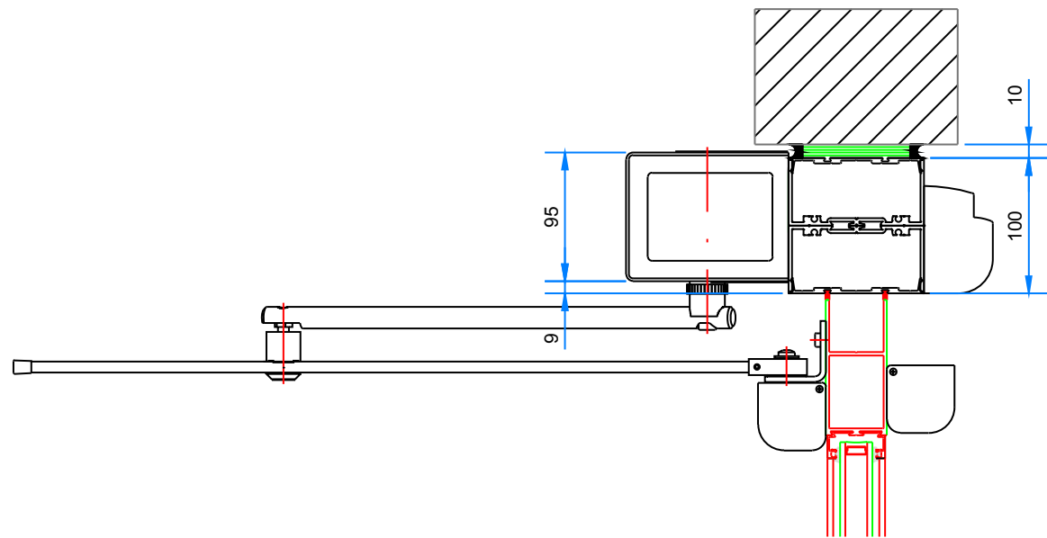
Outswing Rod Push Arm (100mm Section)
